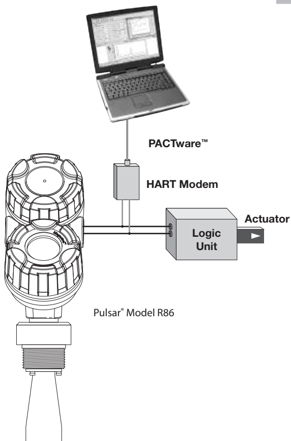
Figure 1 Typical System
